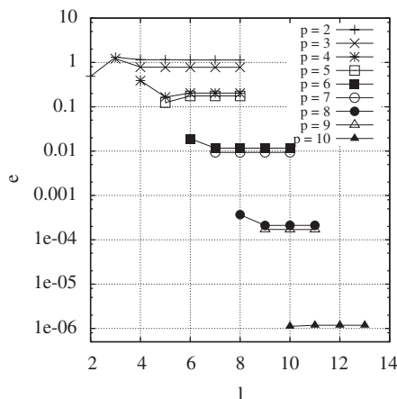
Fig. 2. The left plot shows the errors e on the sensitivity indices computed from the PC expansion using different orders of truncature ( p ) and levels ( l ) for the cubature formula as indicated. The right plot shows the errors e on the sensitivity indices computed from the PC expansion using different rules for the selection of the expansion order p at given level l of the cubature formula.
