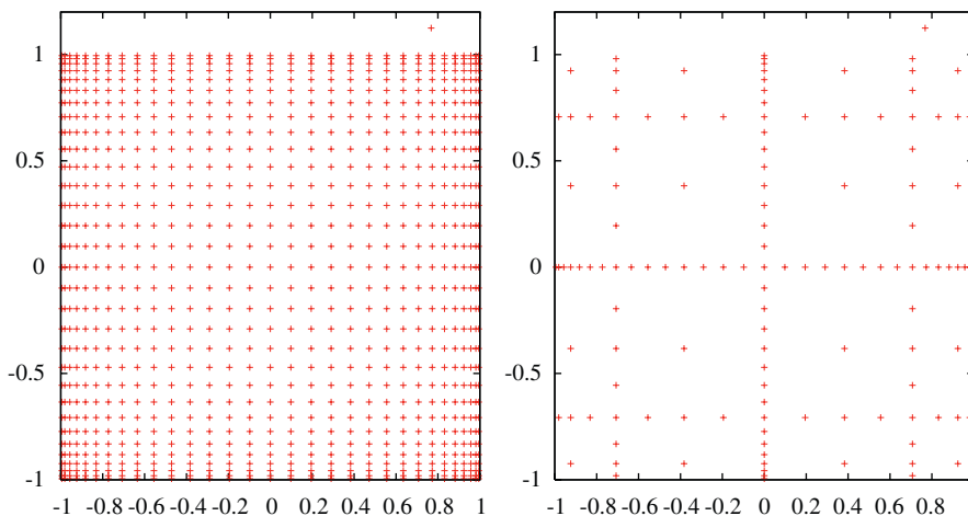
Fig. 1. Quadrature points for the two-dimensional fully tensorized formula (left plot) and two-dimensional Smolyak's partially tensorized formula (right plot). Note that the two formulas have the same degree of exactness for polynomial integrand.
